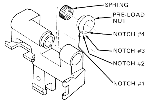
FIGURE 8 CARRIAGE ASSEMBLY
